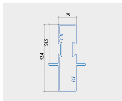
THANH TRUNG GIAN KHUNG BAO
